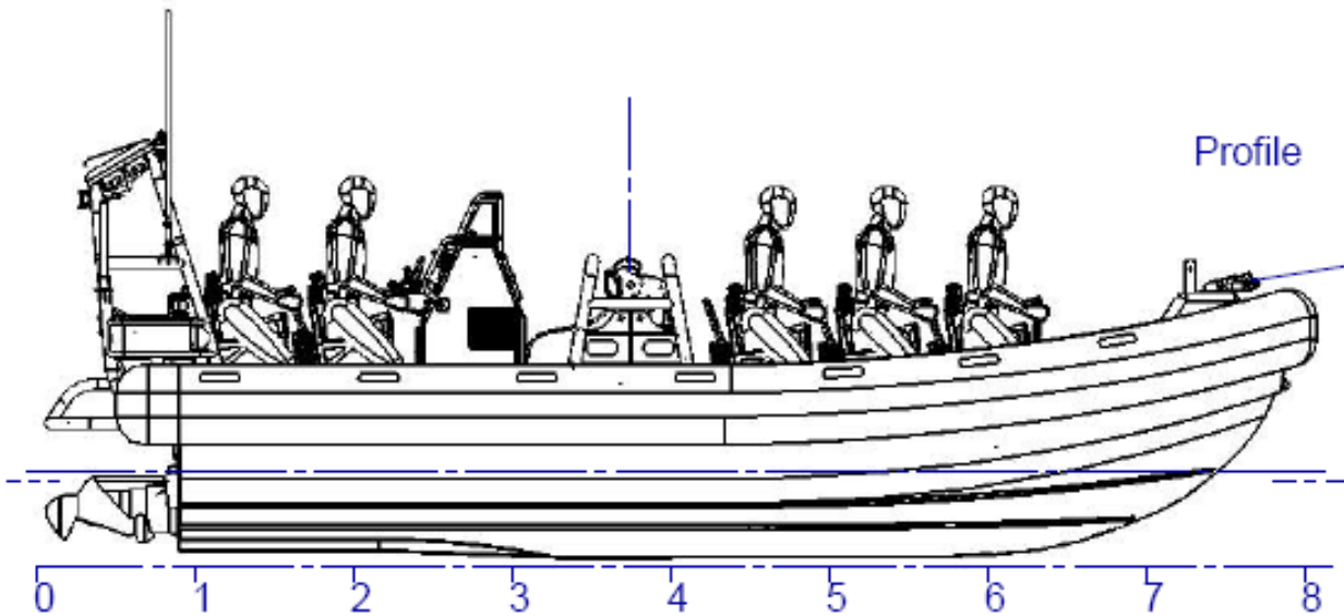
Deck Plan (10 Persons)
